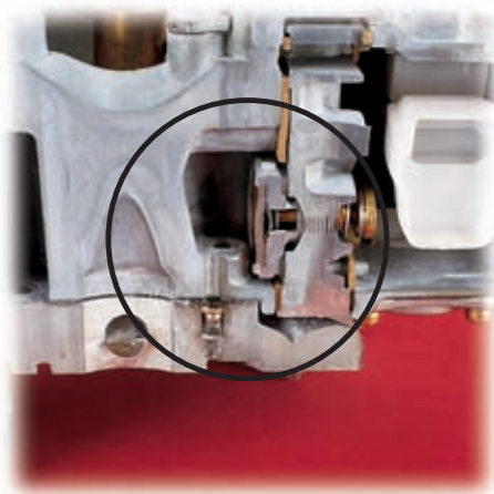
Cut-away of power valve blow-out protection.
