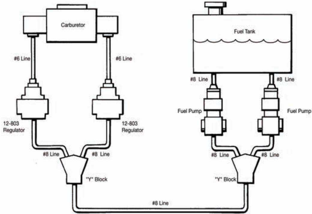
Figure 3 – Two (2) #12-802-1, 12-815-1 or 12-150 “blue” pumps feeding single carburetor.
