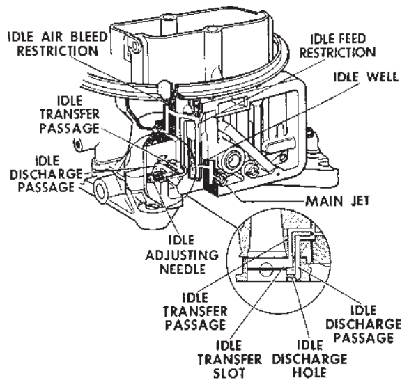
Idle System. Model 2300 — Primary Side 4V.
